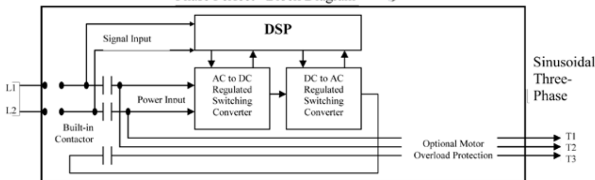
Phase Perfect® Block Diagram
